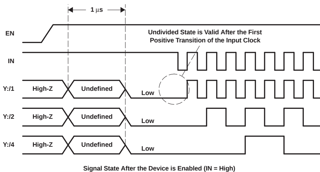
Figure 13. Waveforms
